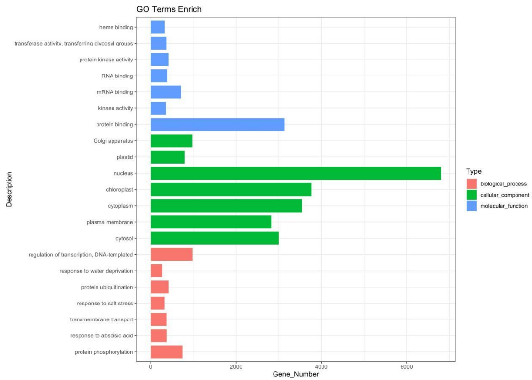
Figure S3. Finger Lemon GO Enrichment Map.
