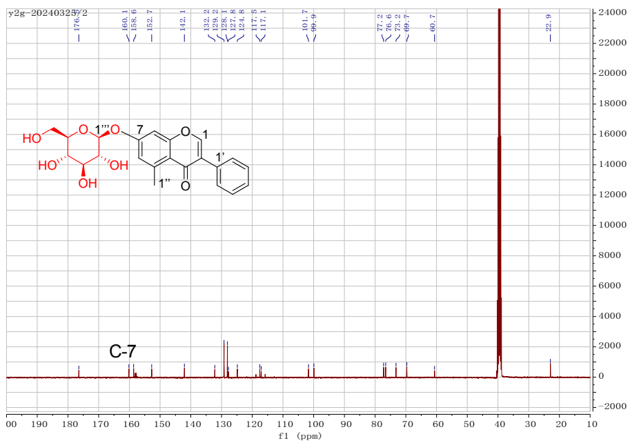
Figure S17. ^{13}\text{C} NMR spectrum of compound 5a in DMSO- d_6 (100 MHz).
