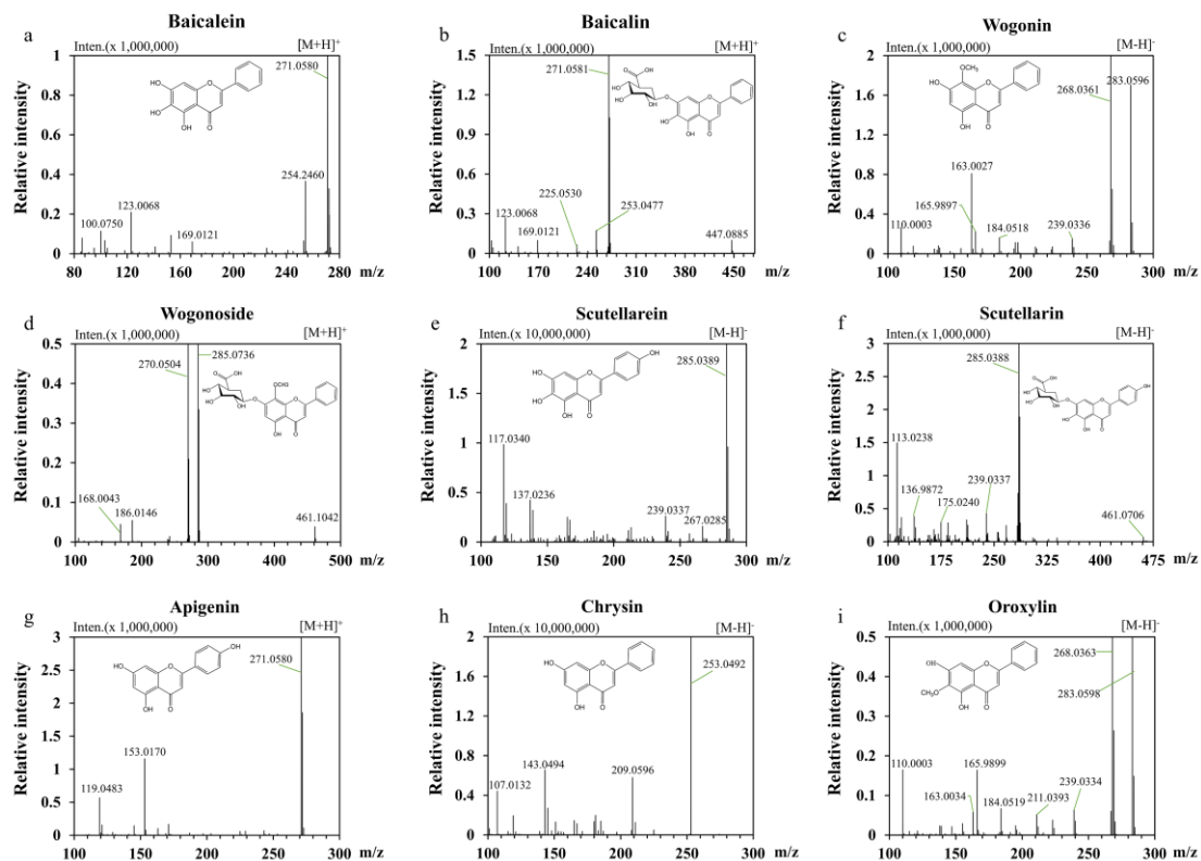
Figure S5. Secondary mass spectrum of nine flavones standard.
