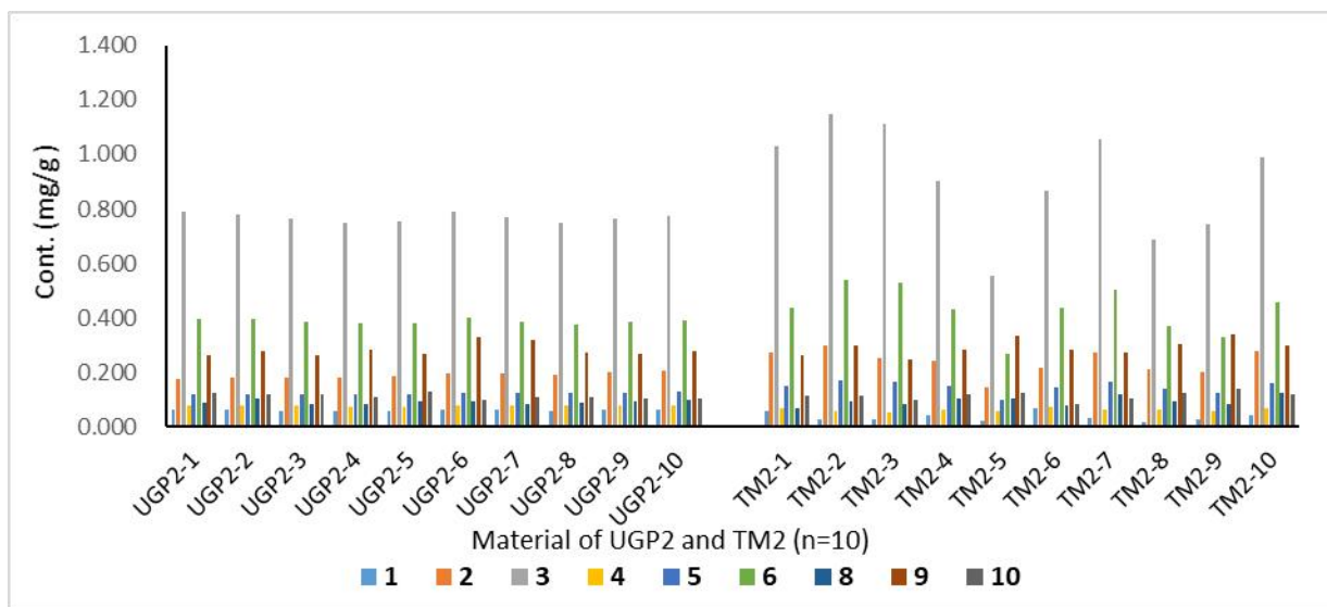
Figure S4. Contents (mg/g) of marker compounds ( 1-6 and 8-10 ) in UGP2 and TM2 from the same source of Astragali Radix (n=10). Marker compounds: calycosin ( 1 ), calycosin-7-O- \beta -D-glucose ( 2 ), calycosin-7-O- \beta -D-glucose-6"-O-malonate ( 3 ), formononetin ( 4 ), ononin ( 5 ), formononetin-7-O- \beta -D-glucoside-6"-O-malonate ( 6 ), astragaloside II ( 8 ), astragaloside I ( 9 ), and acetylastragaloside I ( 10 ).
