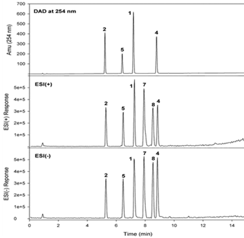
Figure S1. Typical UHPLC-MS-UV chromatograms of six standard compounds.
