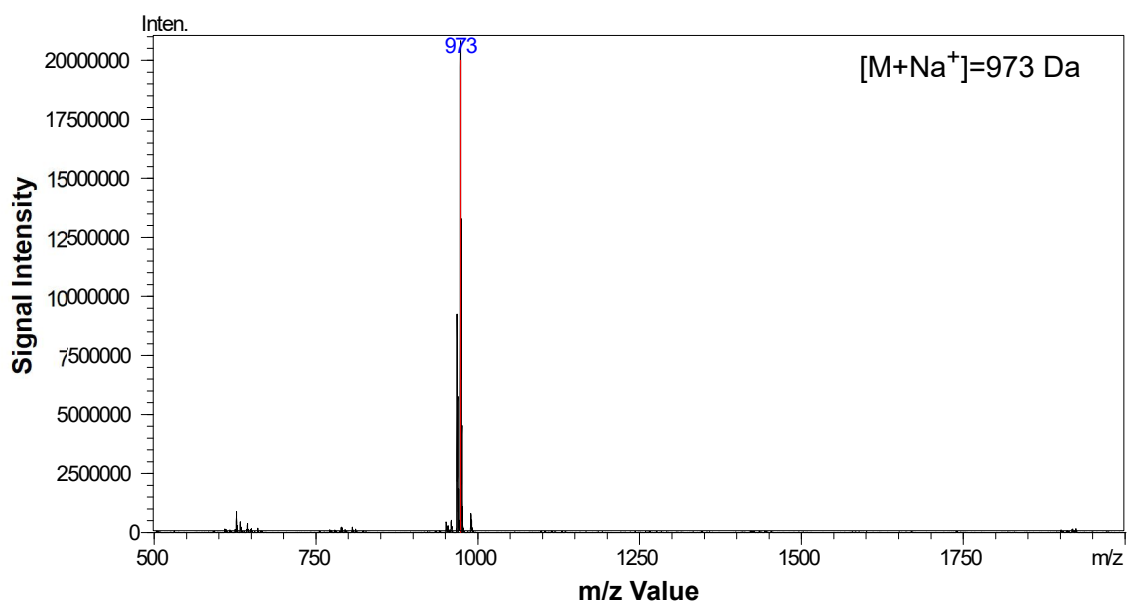
Supplementary Figure S5: LCMS-analysis of Reb C standard. The top panel shows the UV signal ( \lambda=210 nm) with the relevant m/z signal at t-27.3 min (m/z range 500-2000) shown in the bottom panel.
