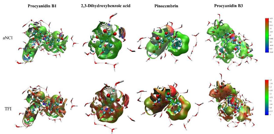
Figure s6. Average noncovalent interaction (aNCI) analysis and thermal fluctuation index (TFI) analysis of procyanidin B1, 2,3-dihydroxybenzoic acid, pinocembrin, and procyanidin B3 in water.
