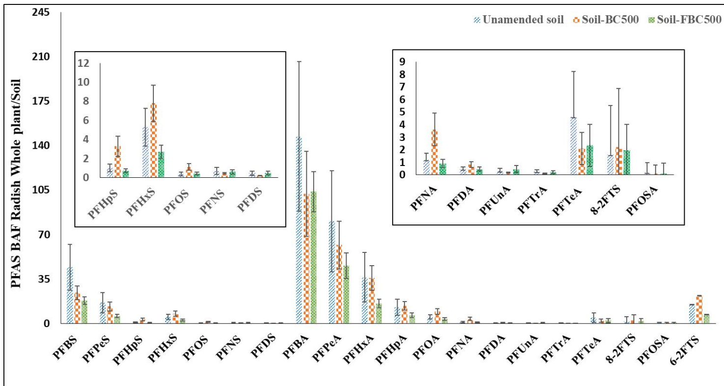
Supplementary Fig. S5. Bioaccumulation factors (BAF) for each PFAS compound in the whole plant grown in contaminated soil with and without sorbent amendments. Error bars represent the standard errors for each treatment ( n = 5 ). Inserts represent magnifications of PFAS compounds with concentrations too low to observe in the main graph.
