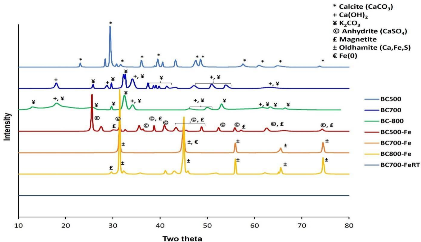
Supplementary Fig. S2 . XRD spectra of the prepared BC sorbents with and without iron fortification at varying pyrolysis temperatures.
