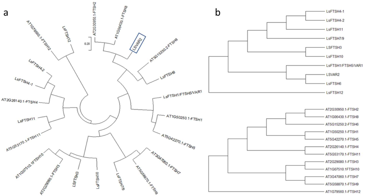
Supplemental Figure 2: Phylogenetic analysis of Arabidopsis and lettuce FtsH genes. (a) Lettuce LsVAR2 is closely related to both FtsH2 and FtsH8; (b) Phylogenetic analysis of FtsH genes in lettuce (top) and in Arabidopsis (bottom).
