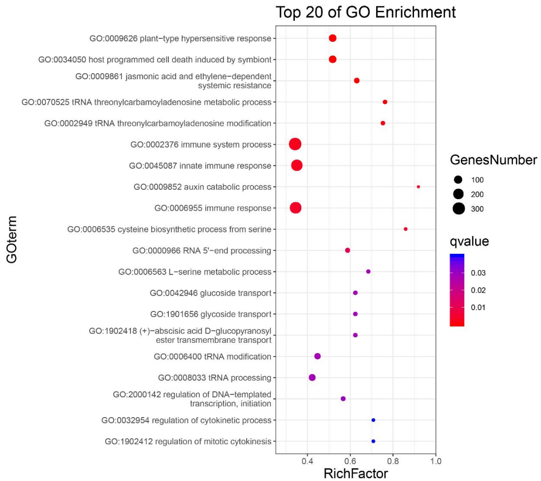
Supplementary Figure 9. GO enrichment analysis(Biological Process) of genes with the SV-overlapping genes.
