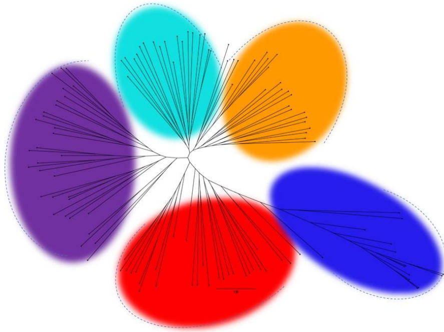
Supplementary Figure 3. Phylogenetic tree based on SNPs, accessions are represented in the same color code throughout this figure (blue=wild, red=Mid, Light purple=SFJ, Teal=NFJ, and Yellow=ZJ).
