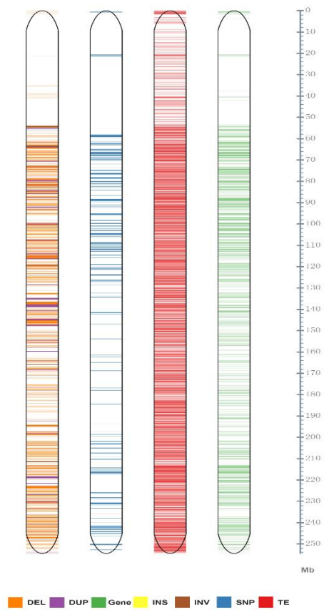
Supplementary Figure 1. Distribution of SVs, gene density and TE density on Chr07.
