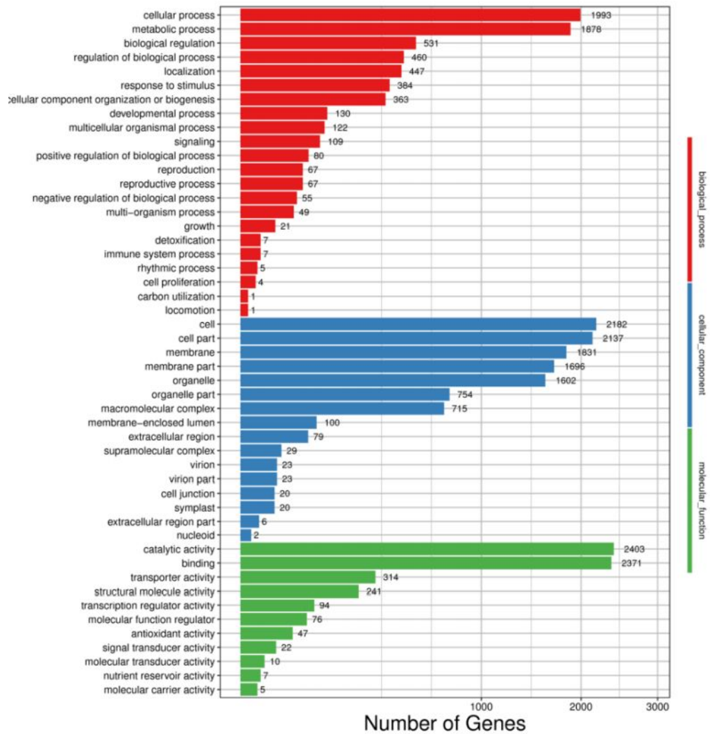
Supplementary Figure 5. GO analysis enrichment of unique gene families in the C. goeringii genome.
