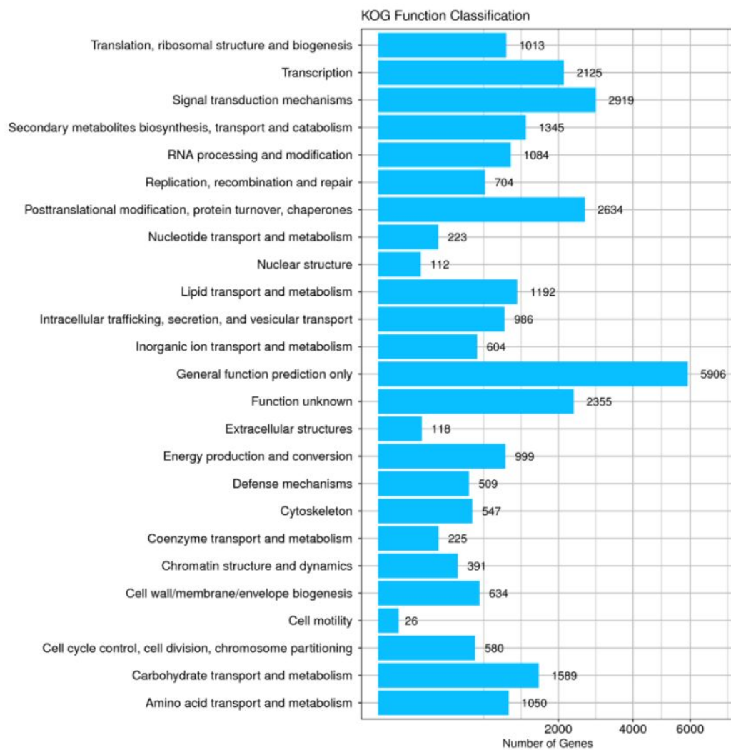
Supplementary Figure 7. KOG pathway enrichment of unique gene families in the C. goeringii genome.
