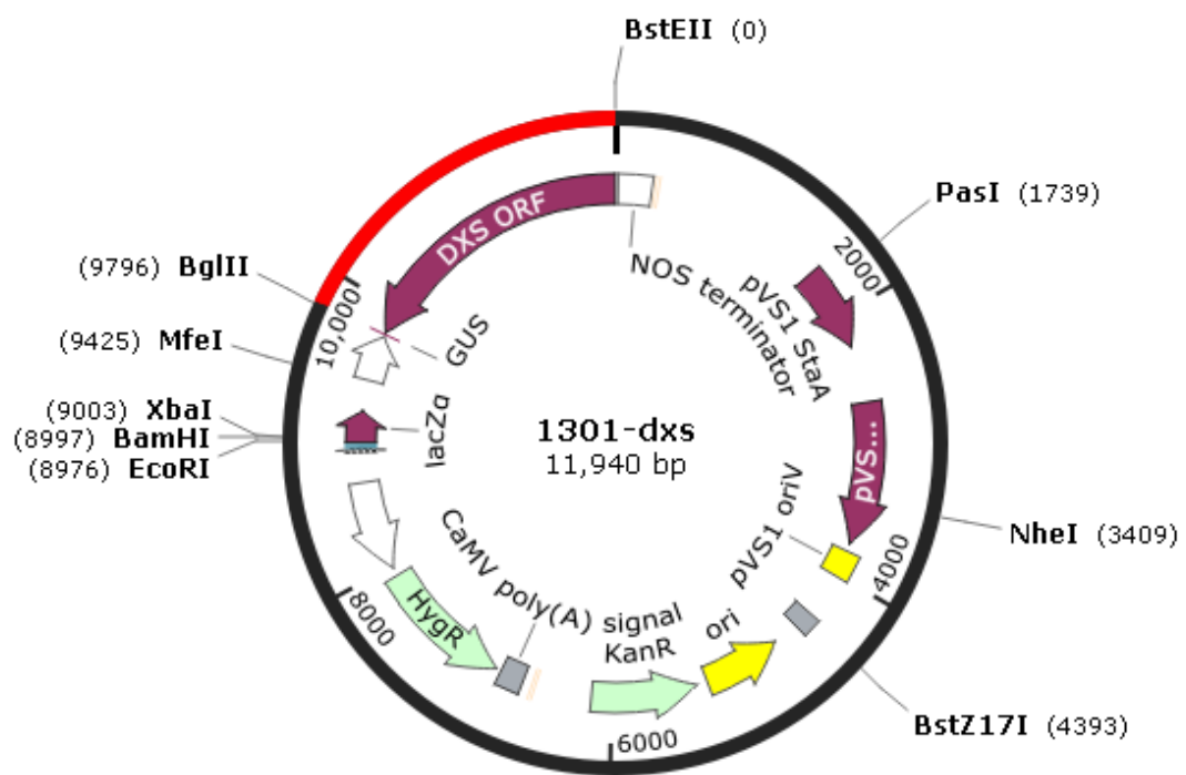
Figure S6 The map of recombinant plasmid pCAMBIA1301-antiDXS1
