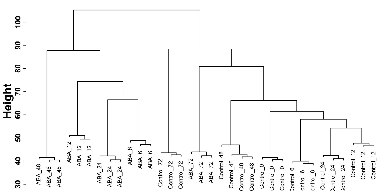
Supplemental Fig. S2 Hierarchical clustering of samples in the deacclimation experiment. All genes after low count filtering were used for clustering.
