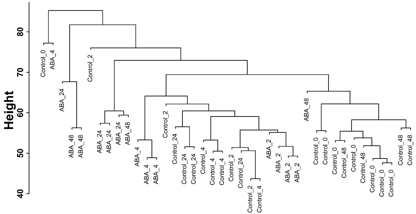
Supplemental Fig. S1 Hierarchical clustering of samples in the acclimation experiment. All genes after low count filtering were used for clustering.
