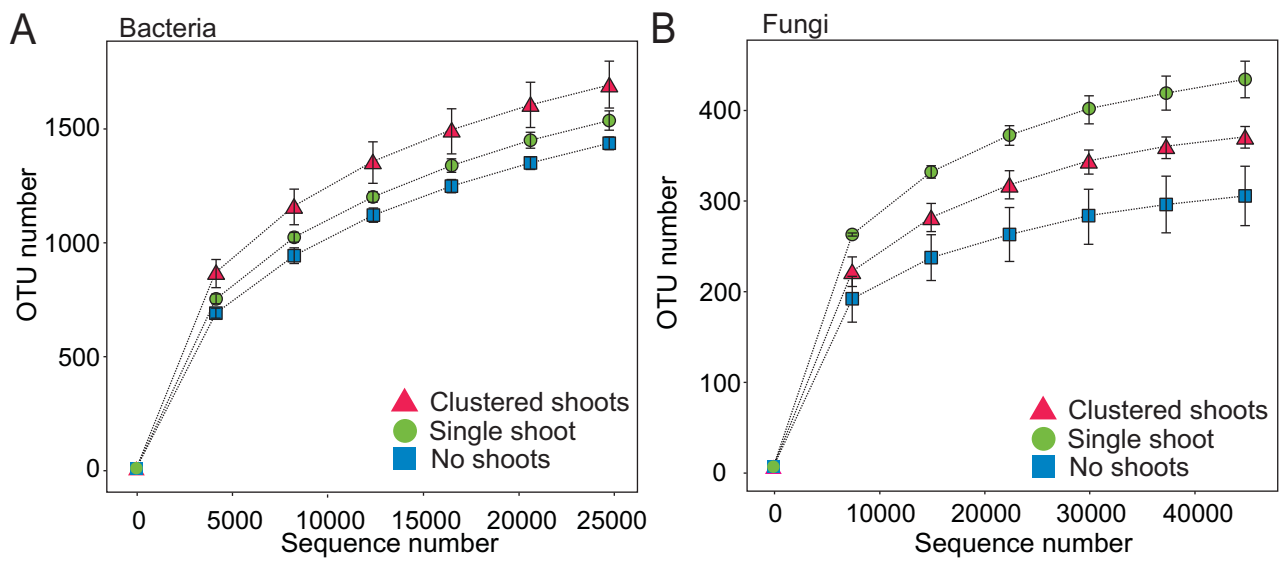
Supplementary Fig. 1. Rarefaction curves of OTUs at 97% similarity for samples from clustered moso bamboo shoots, a single shoot, and no shoots. (A) Bacteria. (B) Fungi. Samples from clustered shoots, a single shoot, and no shoots are indicated by red triangle, green circle, and blue square respectively. The average OTUs number of three samples of each group are shown.
