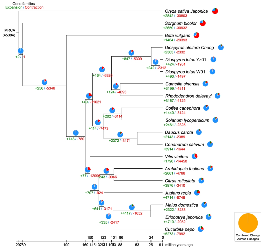
Supplementary Figure S3: Gene family expansion and contraction analysis of 19 species. Green marks the number of expanding genes, and red marks the number of contracting genes.
