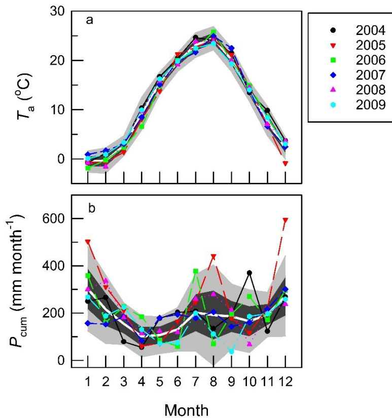
Fig. S2 Monthly mean values of selected meteorological variables recorded at an AMeDAS weather station close to the study sites in 2004-2009. White lines represent 30-year averages (1980-2010) of (a) the mean air temperature ( T_a ) and (b) the monthly precipitation ( P_{cum} ) during the growing season. Dark and light grey areas represent \pm 1 SD and \pm 2 SD, respectively.
