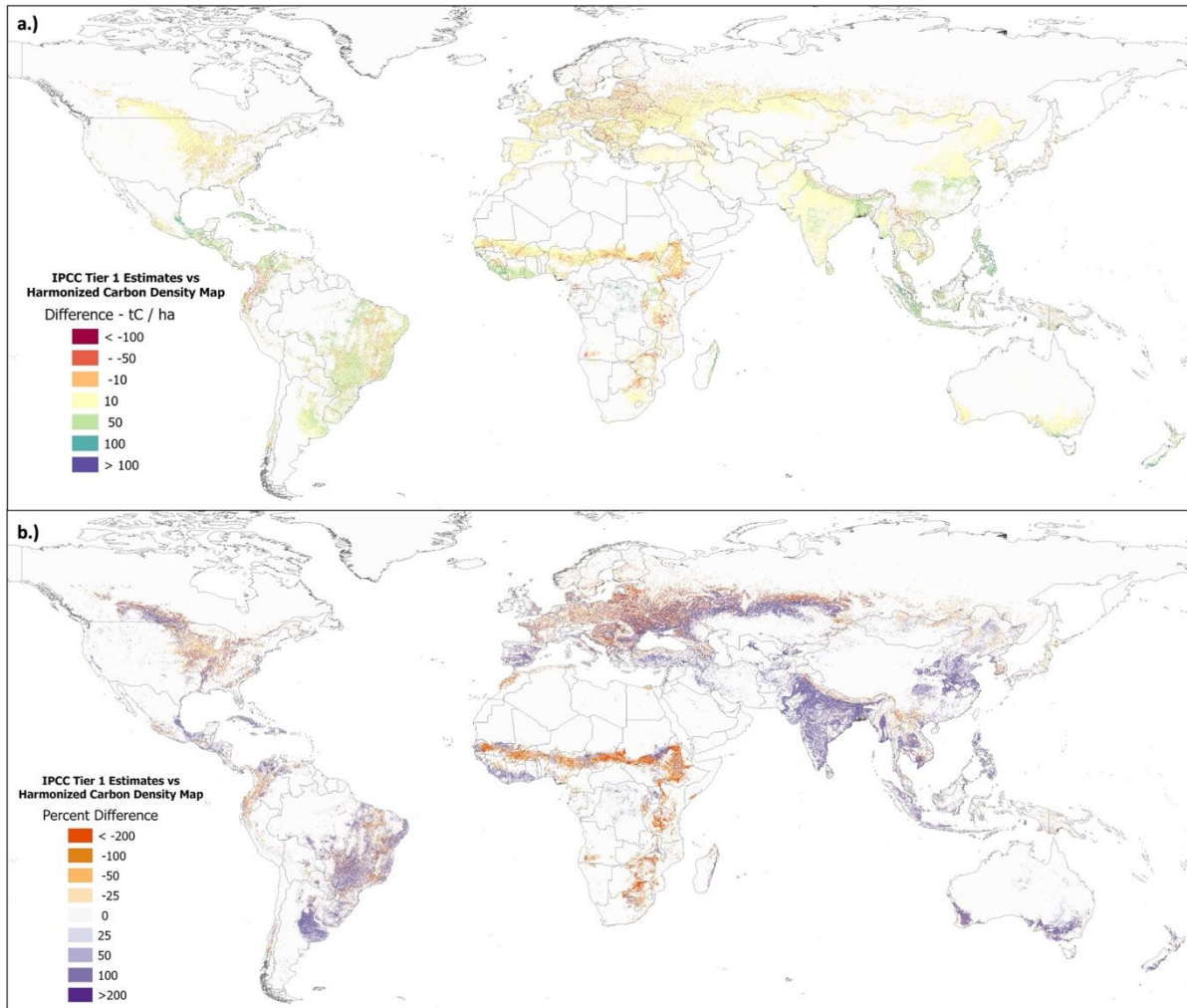
Figure SM_1: Comparison of IPCC Tier 1 based estimates Zomer et al, 2016. vs Harmonized Carbon Density Map Spawn and Gibbs, 2020., a.) showing differences in tC/ha and b.) in percent , with negative values signifying and underestimation by the IPCC Tier 1 based estimates, and positive values an overestimation.
