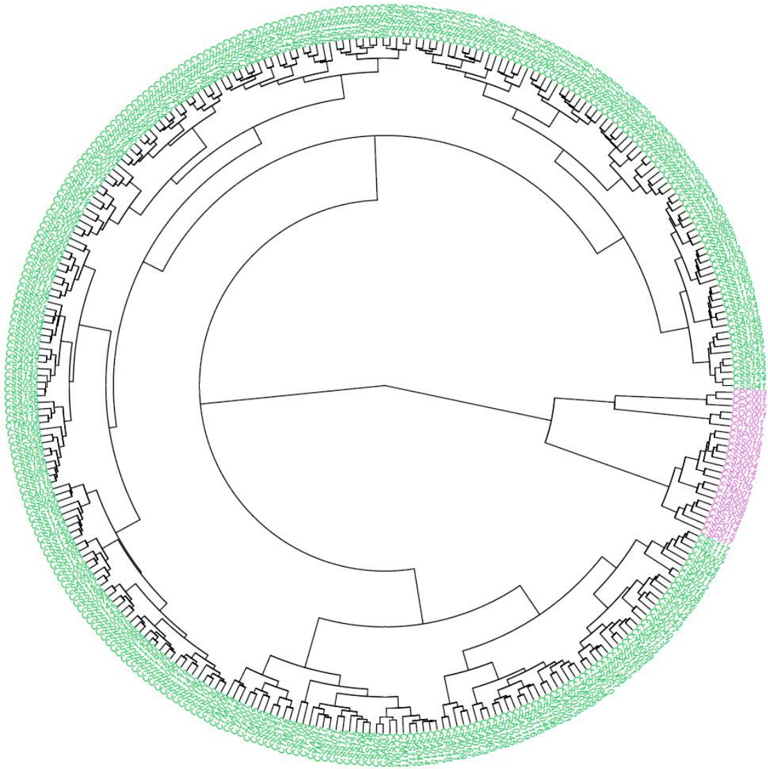
Figure S2 Cluster analysis of the natural population. (Green represents Group 1, purple represents Group 2).
