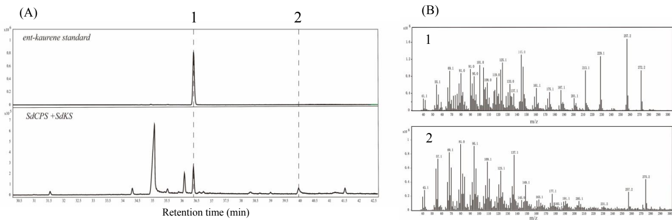
Figure S1. The biochemical activity of SdKS . A, Selective ion chromatograms (BPC=257); B, Mass spectra; 1, ent -kaurene; 2, ent -copalol.
