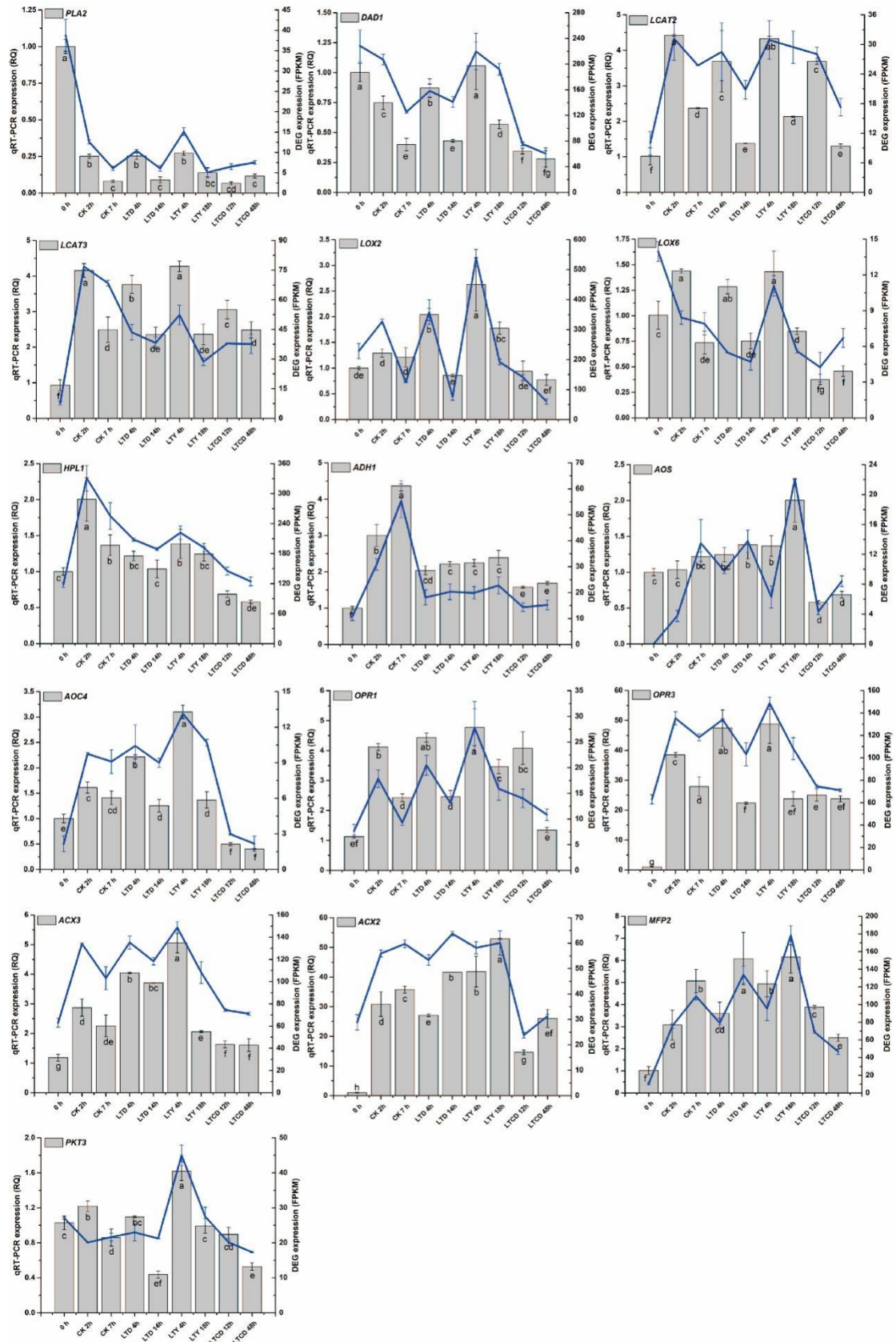
Figure S3. The expression levels of DEGs involved in the catabolic metabolism of \alpha -linolenic acid under different spreading treatments. The different lowercase letters indicate the least significant difference (ANOVA, Duncan test) at p < 0.05 .
