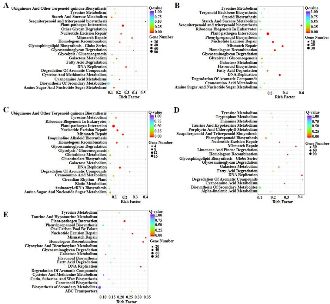
Supplemental Figure S7. The top 20 KEGG pathways enriched by DEGs about Genetic processes, Metabolism and Environmental adaptation compared by the developmental stages of 2F (A), 4F(B), 6F(C), 8F(D) and MF(E) between A161 and R6.
