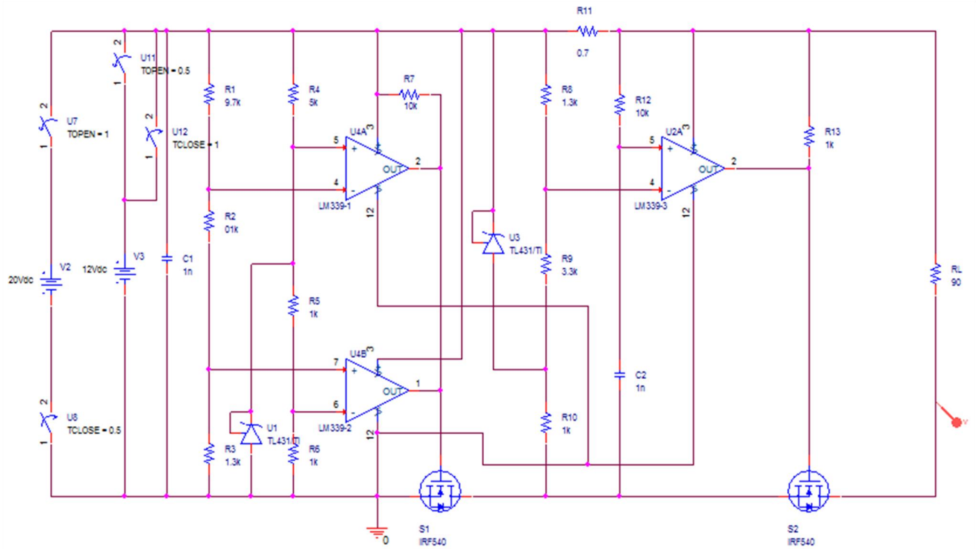
Supplementary Fig. 2 Diagram of undervoltage and overvoltage protection circuit simulation.
