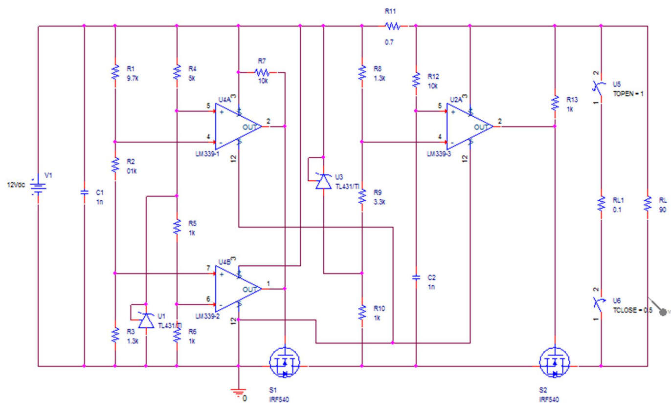
Supplementary Fig. 1 Diagram of overcurrent protection circuit simulation.
