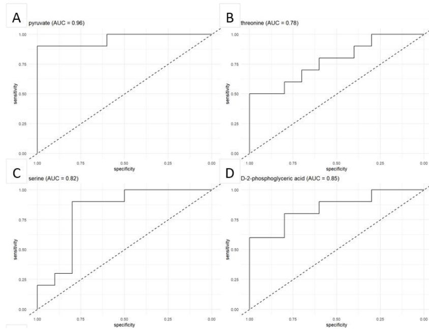
Supplementary Figure S4. ROC curves for key diagnostic metabolites: (A) Pyruvate, (B) Threonine, (C) Serine, (D) D-2-Phosphoglycerate.
