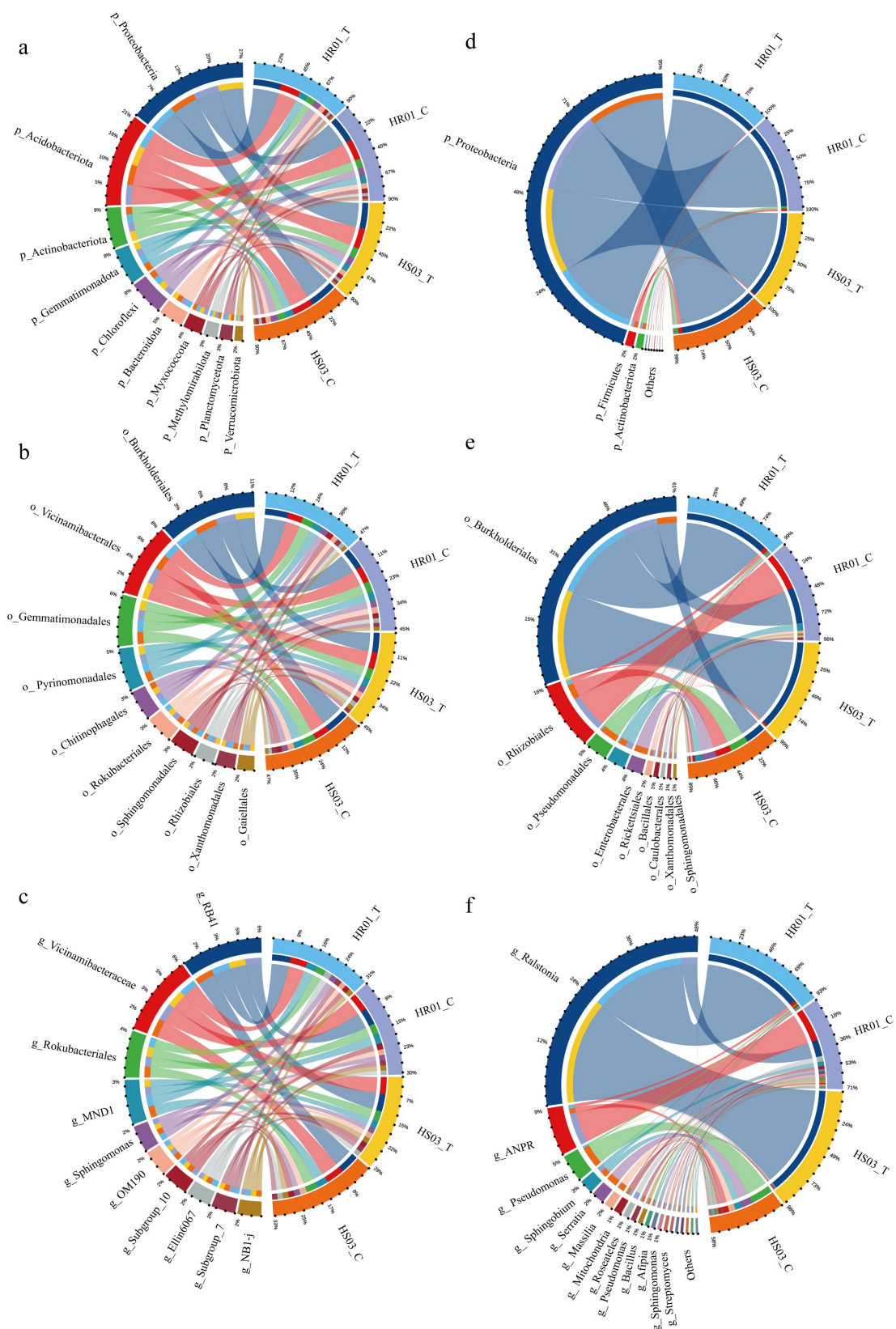
Fig. S1. Community composition of rhizosphere soil (a-c) and roots (d-f) bacterial communities. p: phylum (a, d), o: order (b, e), g: genus (c, f).
