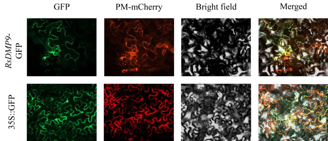
Figure S1. Subcellular localization profiling of RsDMP9. The PM-mCherry was used as a membrane marker. Bars = 50 \mu m.
