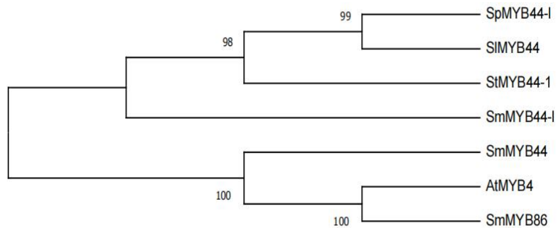
Supplementary Fig. 5 Phylogenetic tree analysis.
