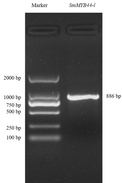
Supplementary Fig. 3 Electropherograms of PCR amplification of the SmMYB44-1 gene.
