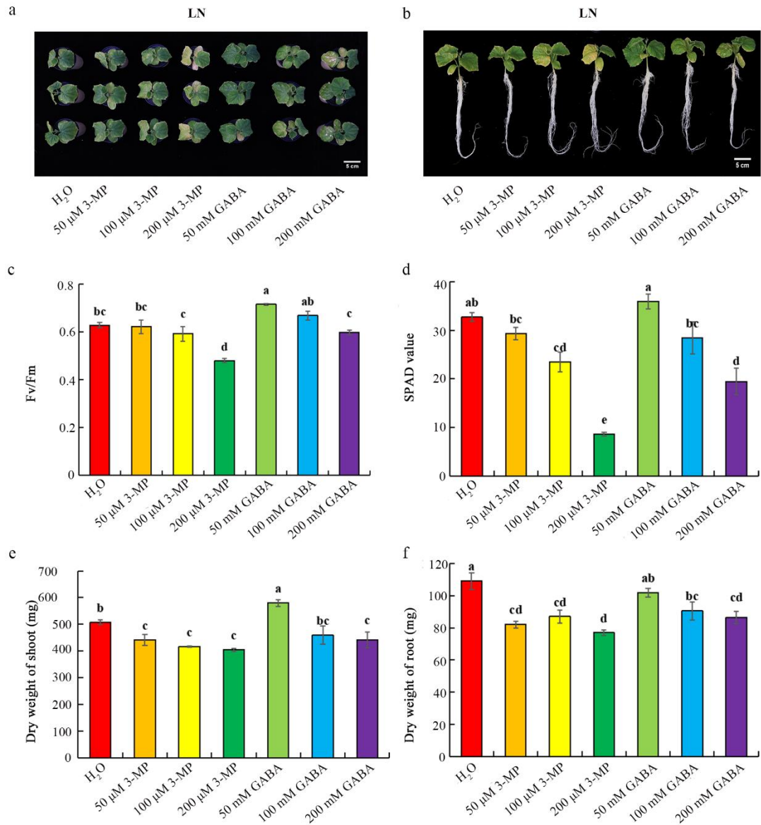
Figure S1. Effects of different concentrations of GABA and its inhibitor 3-mercaptopropionic acid (3-MP) on cucumber accession 9930 under low-nitrogen (LN) conditions.
