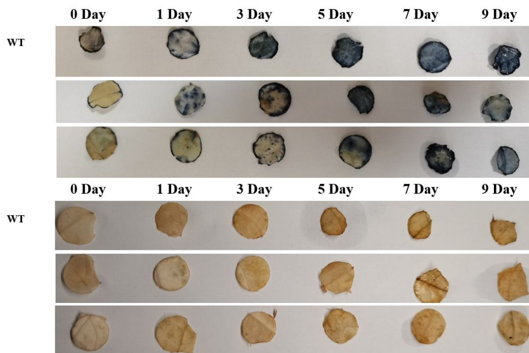
Figure S1. Effects of cold stress on superoxide anion ( O_2^{\bullet-} ) and hydrogen peroxide ( H_2O_2 ) accumulation in eggplant leaves. DAB and NBT staining detection of O_2^{\bullet-} and H_2O_2 levels in eggplant leaves under cold stress ( 5^\circ C , 16h light/8h dark).
