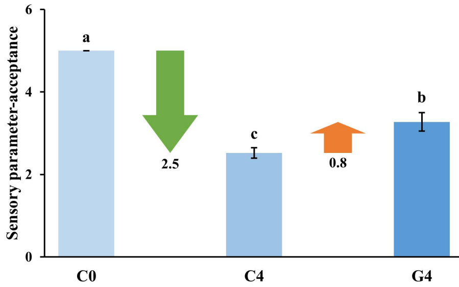
Supplementary Fig. 2 Effects of GABA treatment on sensory parameter-acceptance of baby mustard during postharvest storage.
