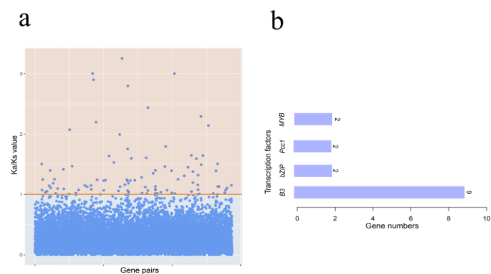
Fig. S5. The identification of positively selected genes and expression patterns of positively selected transcription factors in the watercress genome. a. The Ka/Ks distribution dot plot of homologous gene pair. b. The positively selected transcription factors numbers.
