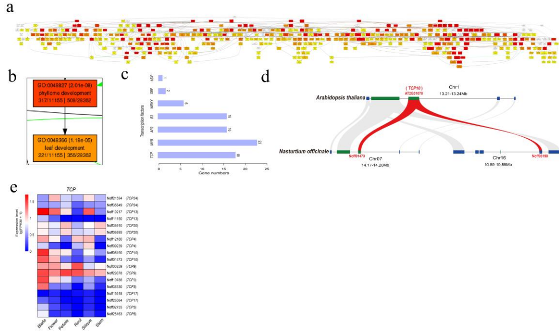
Fig. S4 The analysis of gene retention of WGD. a. The functional pathway annotation plot of homologous Arabidopsis thaliana gene aligned with retained gene after WGD in Nasturtium officinale . b. The specific presentation of homologous Arabidopsis thaliana gene related to leaf development. c. The distribution of transcription factor numbers related to leaf development in Nasturtium officinale . d. The example of gene retention after WGD ( TCP10 ). e. The expression patterns of TCP transcription factors.
