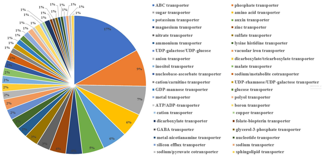
Figure S4 Pie Graph showing the DEGs in Se0 vs Se40 annotated as different transporters in NR database. The proportions of different transporters were presented.
