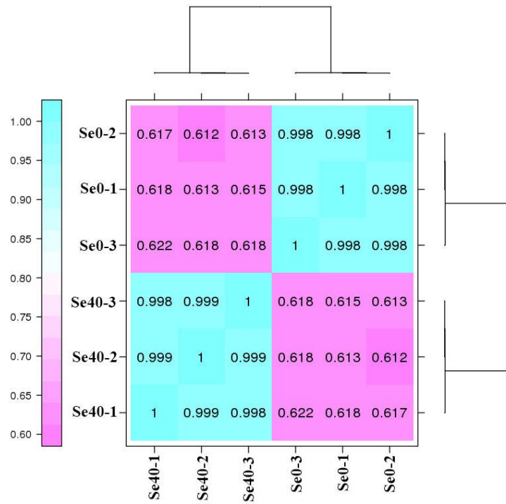
Figure S2 Pearson's correlation coefficients (R) between the three biological replicates of each sample.
