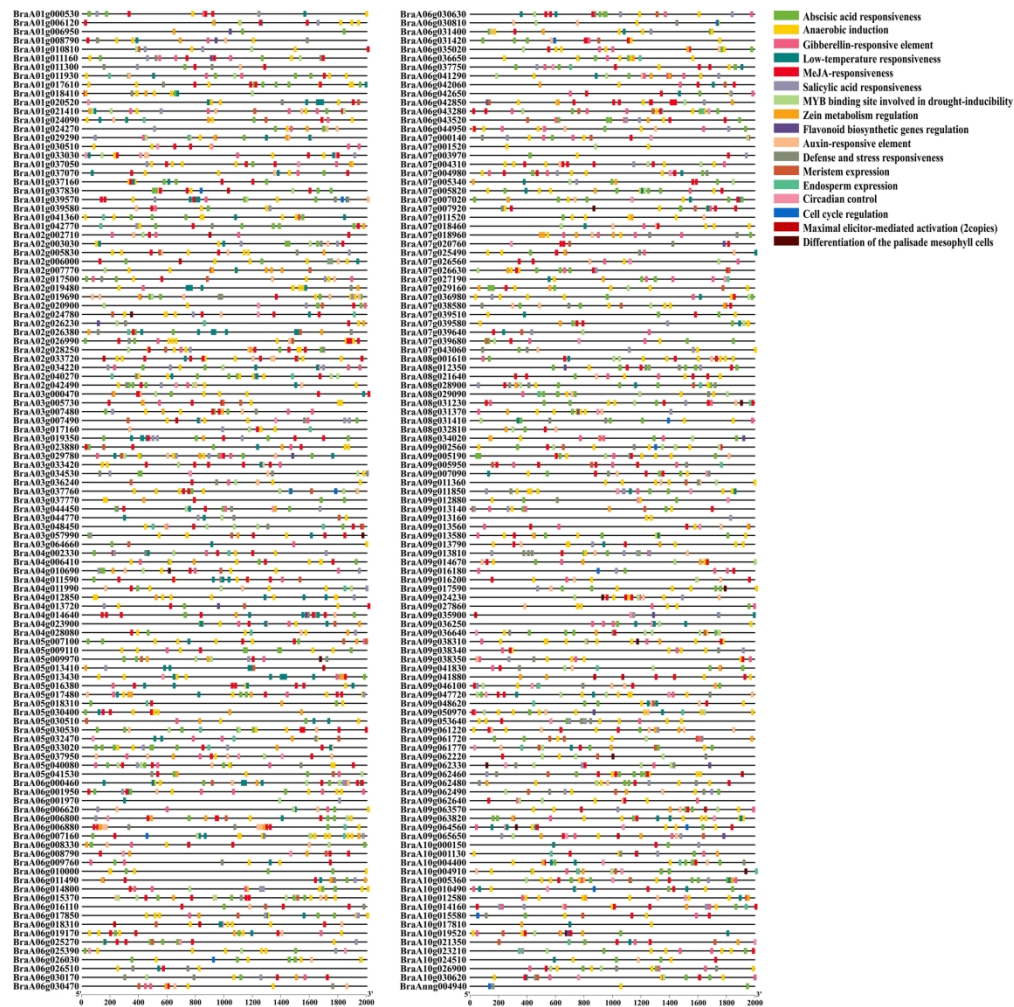
Fig. S6 Cis-acting element analysis of the promoter regions in the P subfamily genes.
