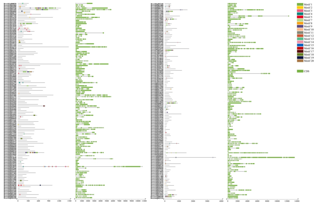
Fig. S3 Structural characteristics and motif distribution of PLS subfamily genes.
