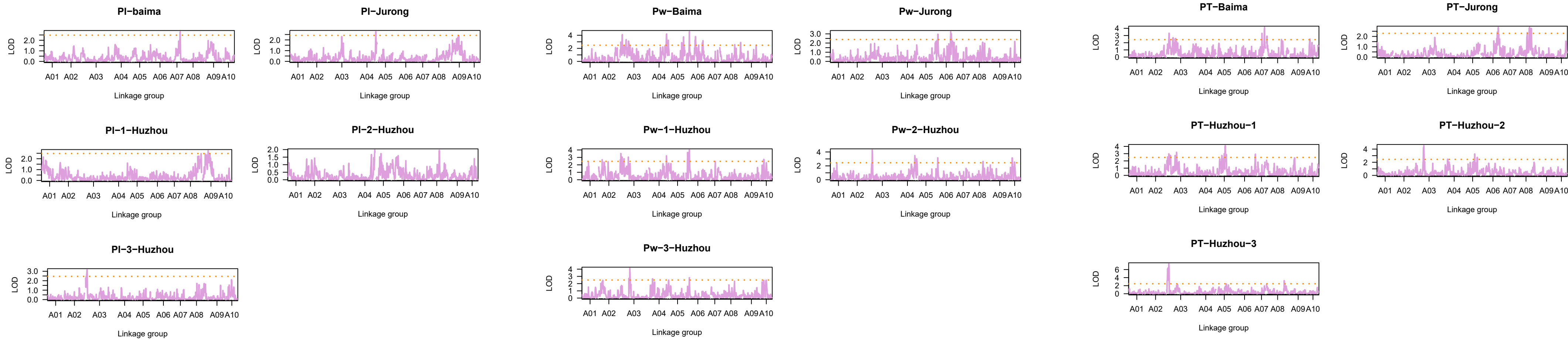
Fig. S2 The QTL for PL, PW, and PT collected from three locations
