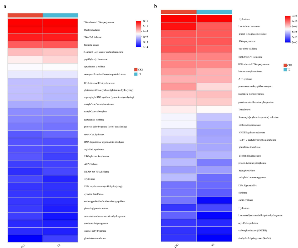
Figure S5 The functional heatmap predicted by PICRUSt2 in bacteria (a) and fungi (b) in CK1 and T2.
