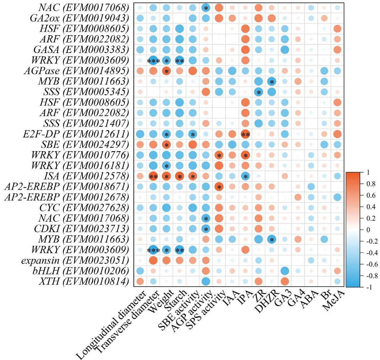
Figure S5 The correlation analysis of taro cormel phenotype, starch content and phytohormone levels between candidate gene expression levels. The Pearson correlation coefficients are colored in red and blue for high and low coefficient between two indexes. The cycle size represented the significance level. * indicates that the coefficients were significantly enriched at 0.05 level. ** indicates that the coefficients were significantly enriched at 0.01 level. *** indicates that the coefficients were significantly enriched at 0.01 level.
