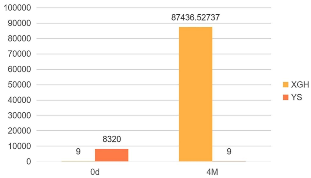
Figure. S1 Changes in the abundance of hydroperoxylinoleic acid in XGH-0d vs. XGH-4M and YS-0d vs. YS-4M.
