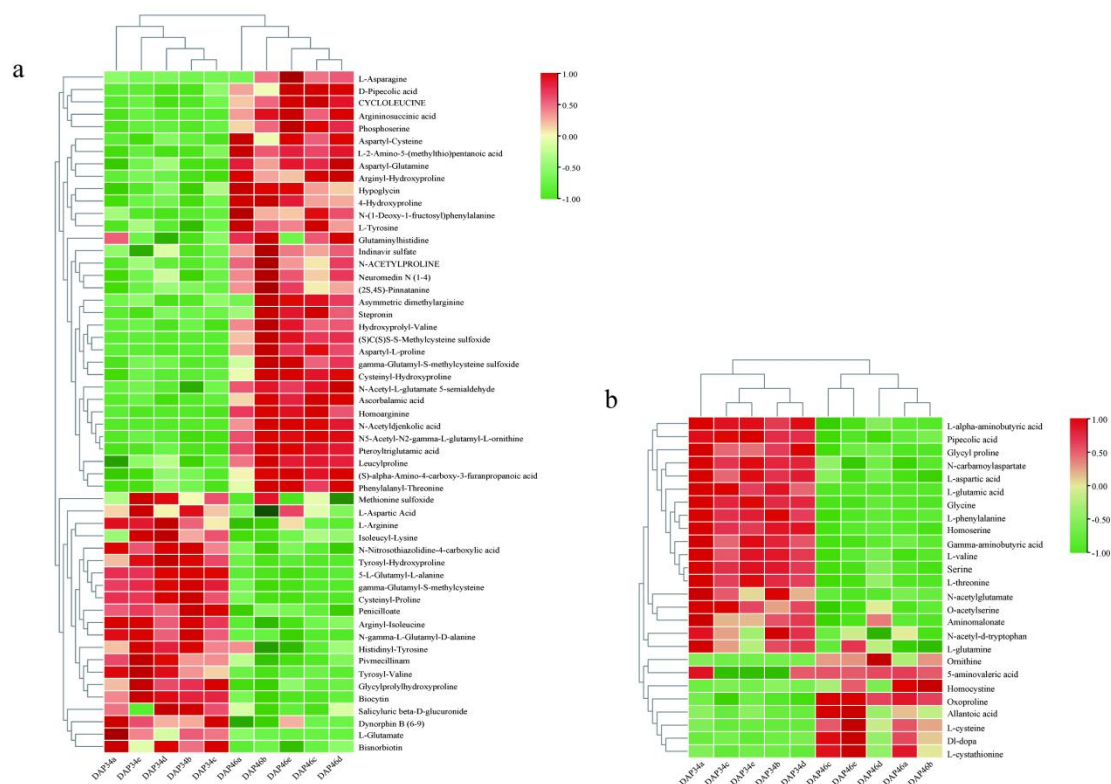
Fig S2. Heat maps of amino acids, polypeptides, and analogues detected by (A) LC-MS/MS and (B) GC-MS/MS.
