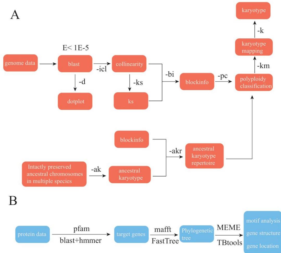
Supplementary Figure 13. Flowchart of the ancestral karyotype construction of the Caryophyllales. The pink blocks represent the various modules used in the WGD software, and the black text indicates the parameters used for each module.
