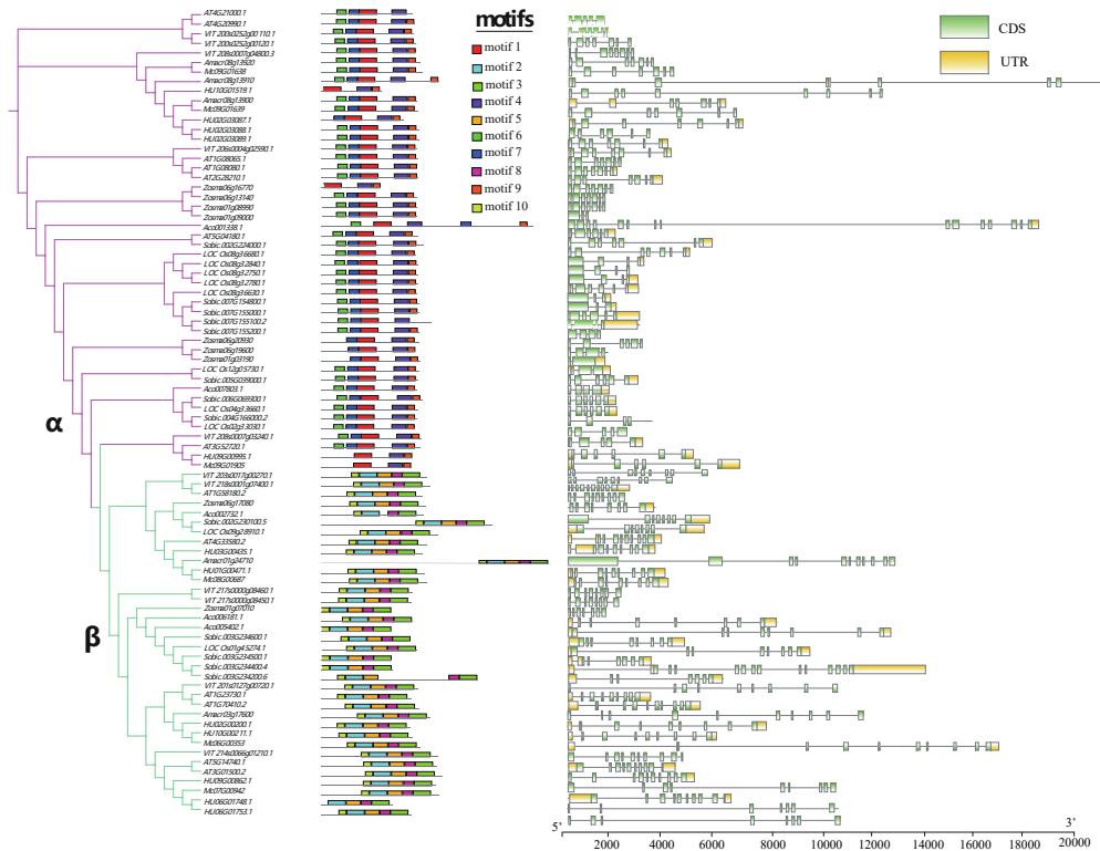
Supplementary Figure 6. Phylogenetic tree, conserved motifs and gene structure of ice plant and other species carbonic anhydrases. On the left-hand side of the dendrogram, schematic depictions elucidate the conserved motifs present within CA proteins, as discerned through the utilization of MEME. These representations employ a diverse palette of colors, each corresponding to a distinct motif identified within the CA protein sequences. On the right side of the dendrogram, schematic illustration delineates the gene architecture characteristic of CA proteins, rendered through TBtools. The green hues demarcate CDS and the yellow demarcate UTR.
