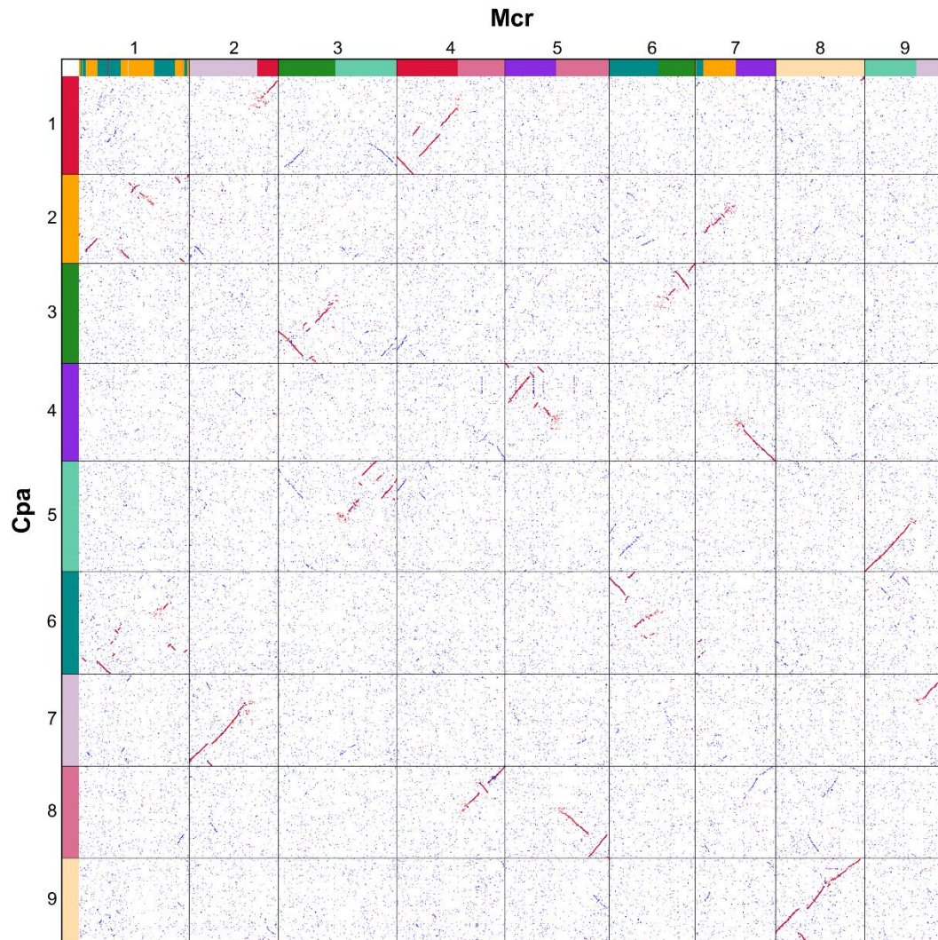
Supplementary Figure 3. The Homologous dotplots between Chenopodium pallidicaule and Mesembryanthemum crystallinum . The numbers in the dotplot represent the chromosome numbers attributed to each respective species under consideration. Red fragments serve to represent optimal alignment between species, while blue segments indicate the secondary levels of correspondence. The line segments composed of red dots in the dotplot do not overlap in the horizontal and vertical directions, which reflects that the ratio of the best-matched homologous regions is 1:1.
